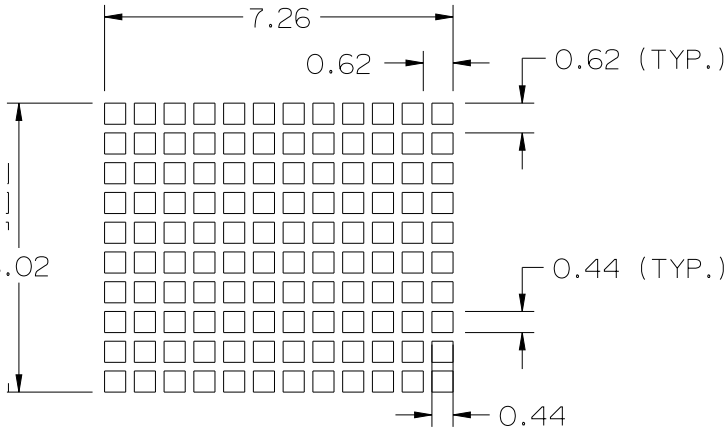
VIEW A TYPICAL VENT PATTERN 0.44 SQ. HOLES (10) VERT. X (12) HORZ.
